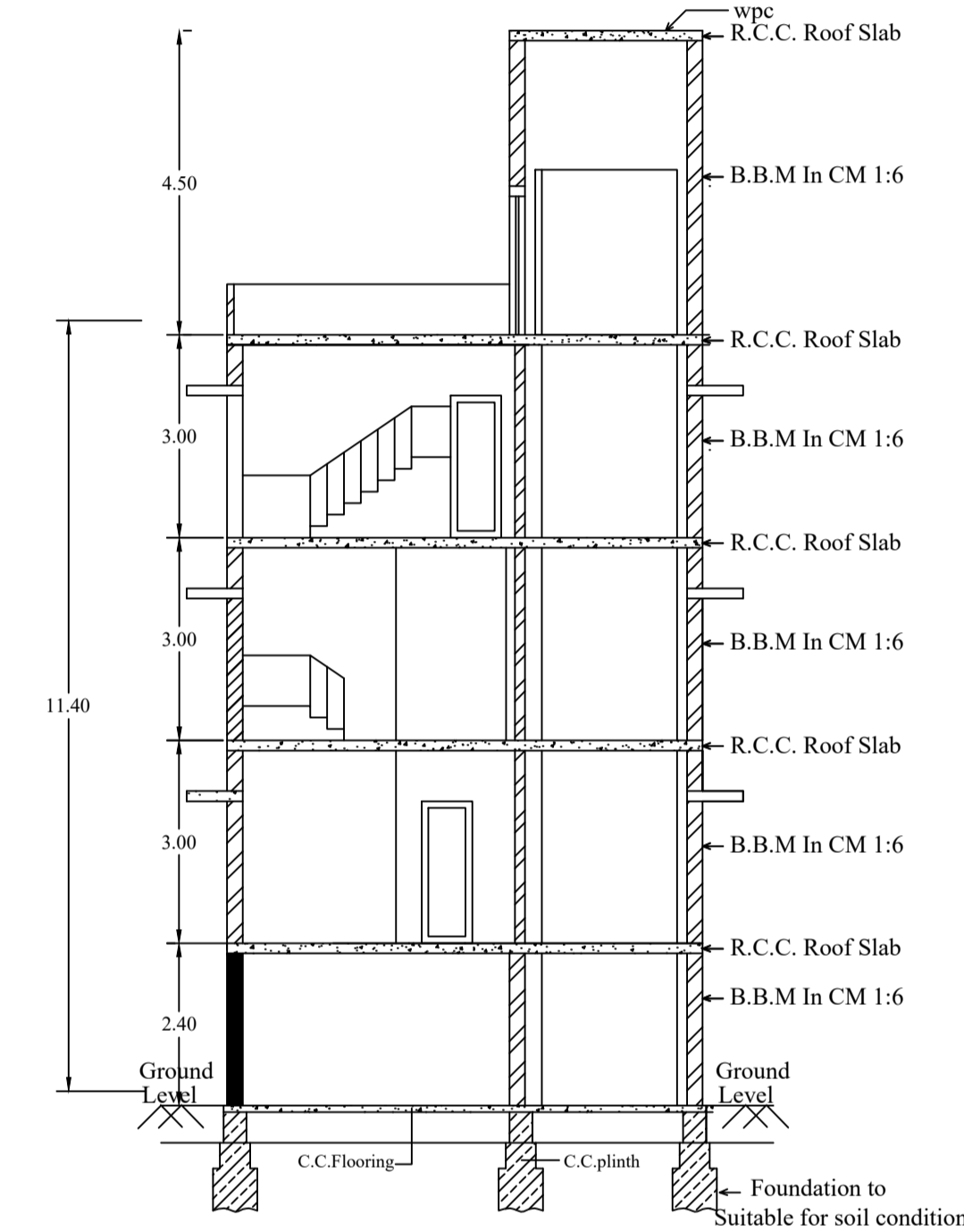
SECTION @ X-X
